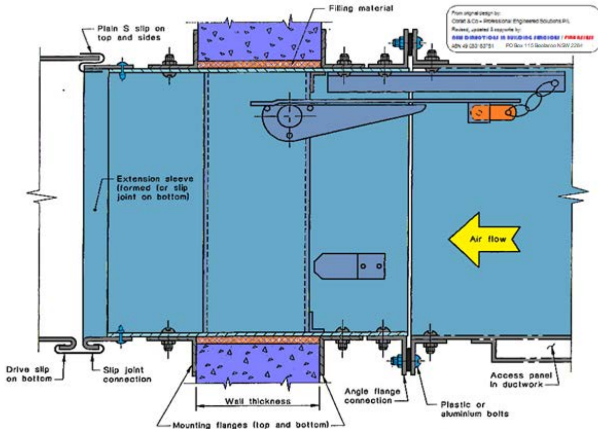
FIGURE B2 TYPICAL FIRE DAMPER INSTALLATION WITH 'BREAKWAY' DUCT CONNECTION
